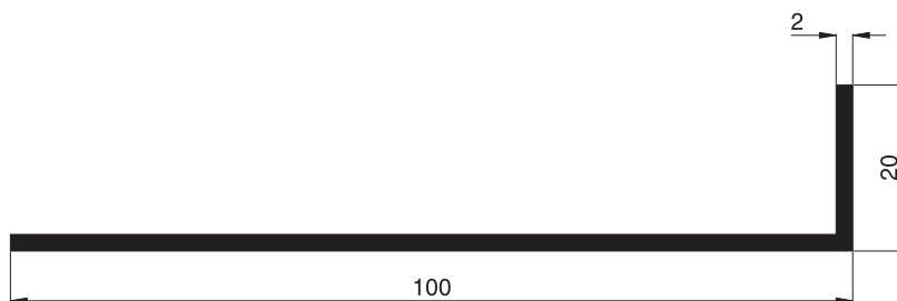
10 91 40 Winkelprofil 100/20/2
